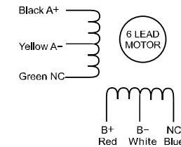
Figure 5: 6-lead motor half coil (higher speed) connections
