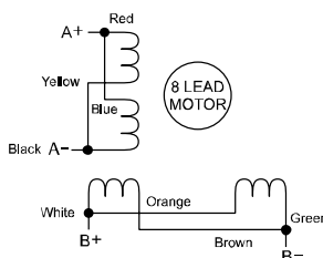
Figure 8: 8-lead motor parallel connections
