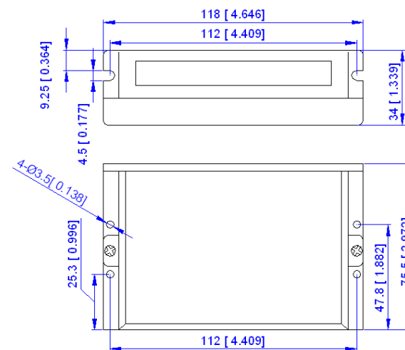
Figure 1: Mechanical dimensions
