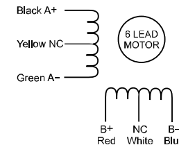
Figure 6: 6-lead motor full coil (higher torque) connections
