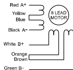
Figure 7: 8-lead motor series connections
