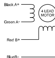
Figure 4: 4-lead Motor Connections
